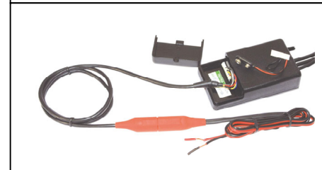
Part 155. (PSU-M4) Power lead (Part A of a two part power lead) For a remote mounted (tank-bag) Pro-7-Sport. MUST be used with either part 156, 134 or 135. (shown plugged into Pro-7-Sport & part 156)
