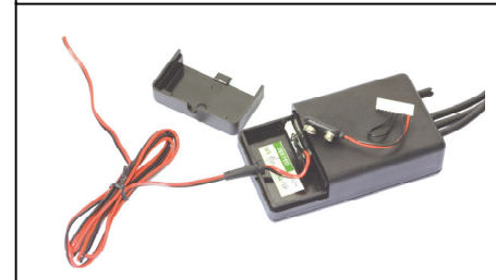
Part 152. (PSU-M2) 12 volt power lead for a bike mounted Pro-7-Sport (shown plugged into Pro-M1)
